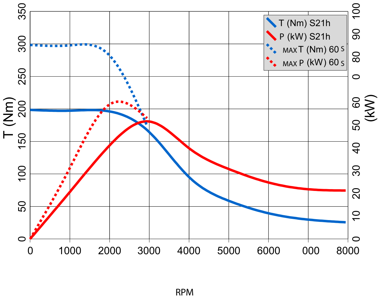
EVE M3-AC40/4-L 40kW 240Vdc
